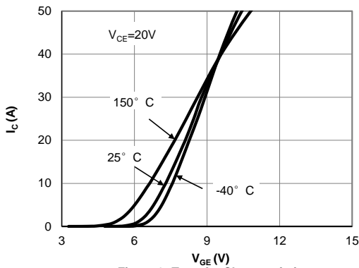
Figure 3: Transfer Characteristic
