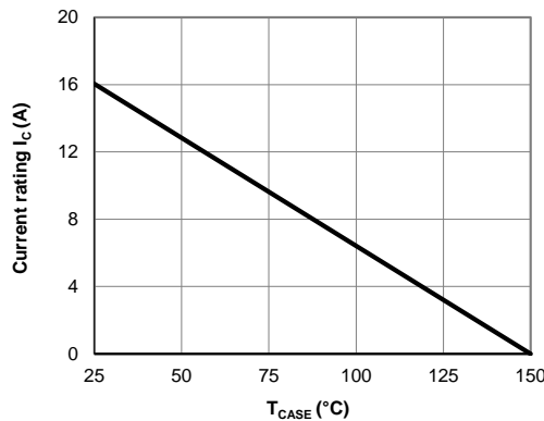
Figure 11: Current De-rating
