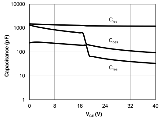
Figure 8: Capacitance Characteristic
